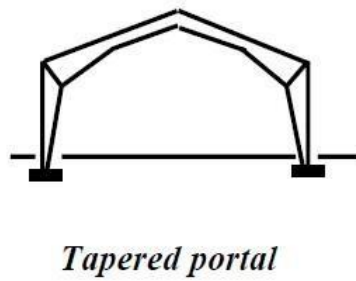
Figure 2.1 Examples of steel frame structure
