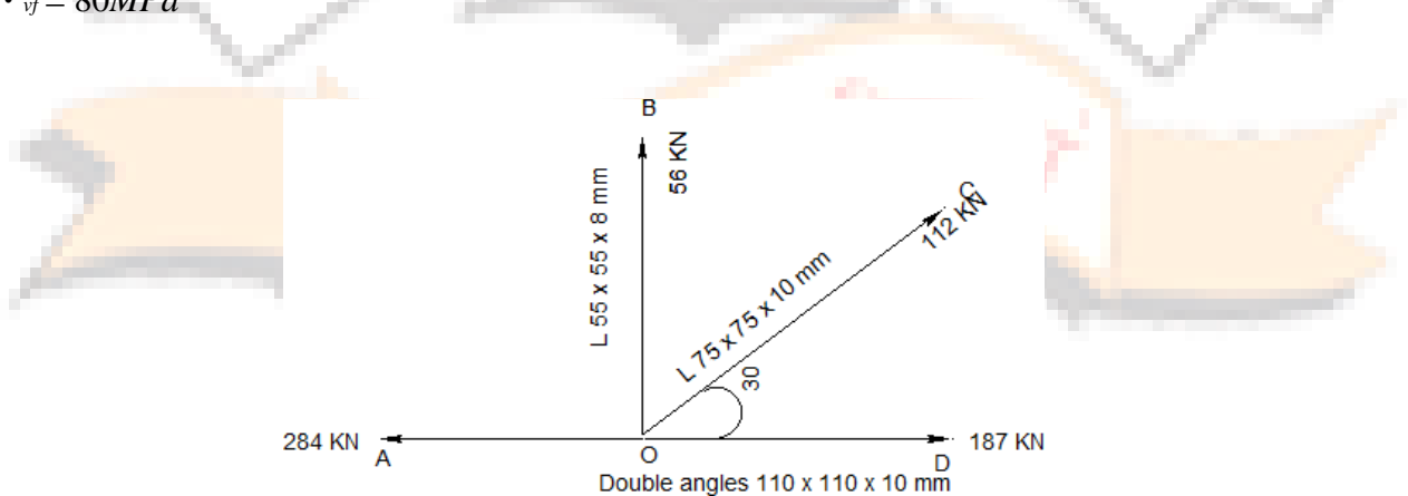
Figure 6.4 A truss joint
