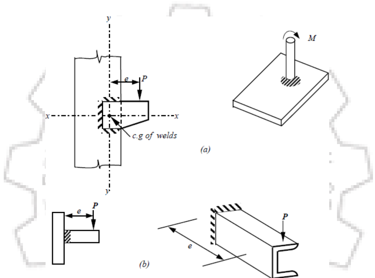
Figure 8.14 (a) Welds subjected to shear and torsion, (b) Welds subjected to shear and bending
