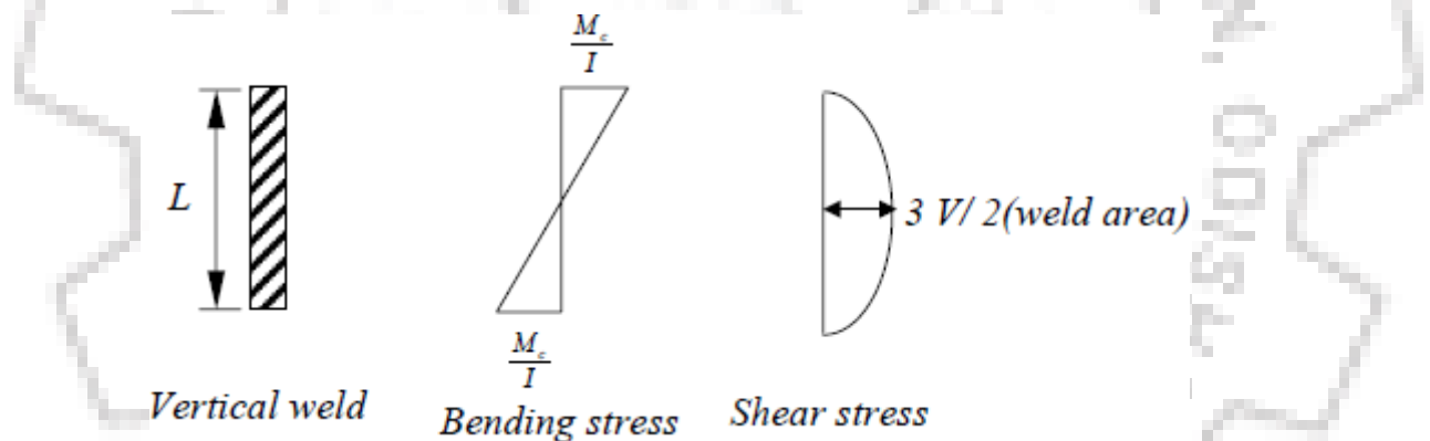
Figure 8.15 Variation of bending and shear stress
