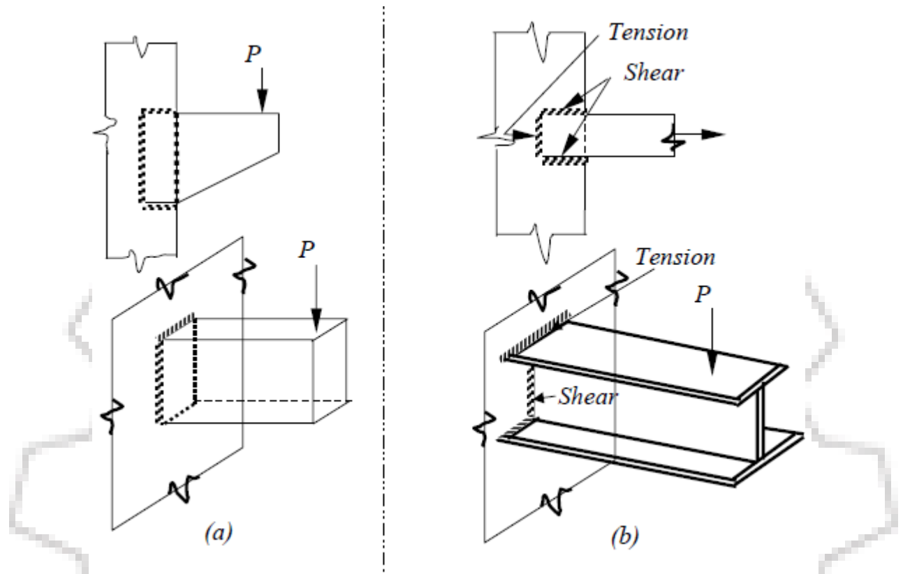
Figure 8.9 (a) connections with simple weld design,(b) connections with direction- dependent weld design
