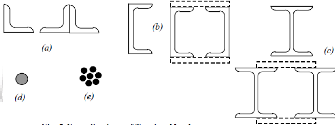
Figure 9.2 Cross section of tension members
