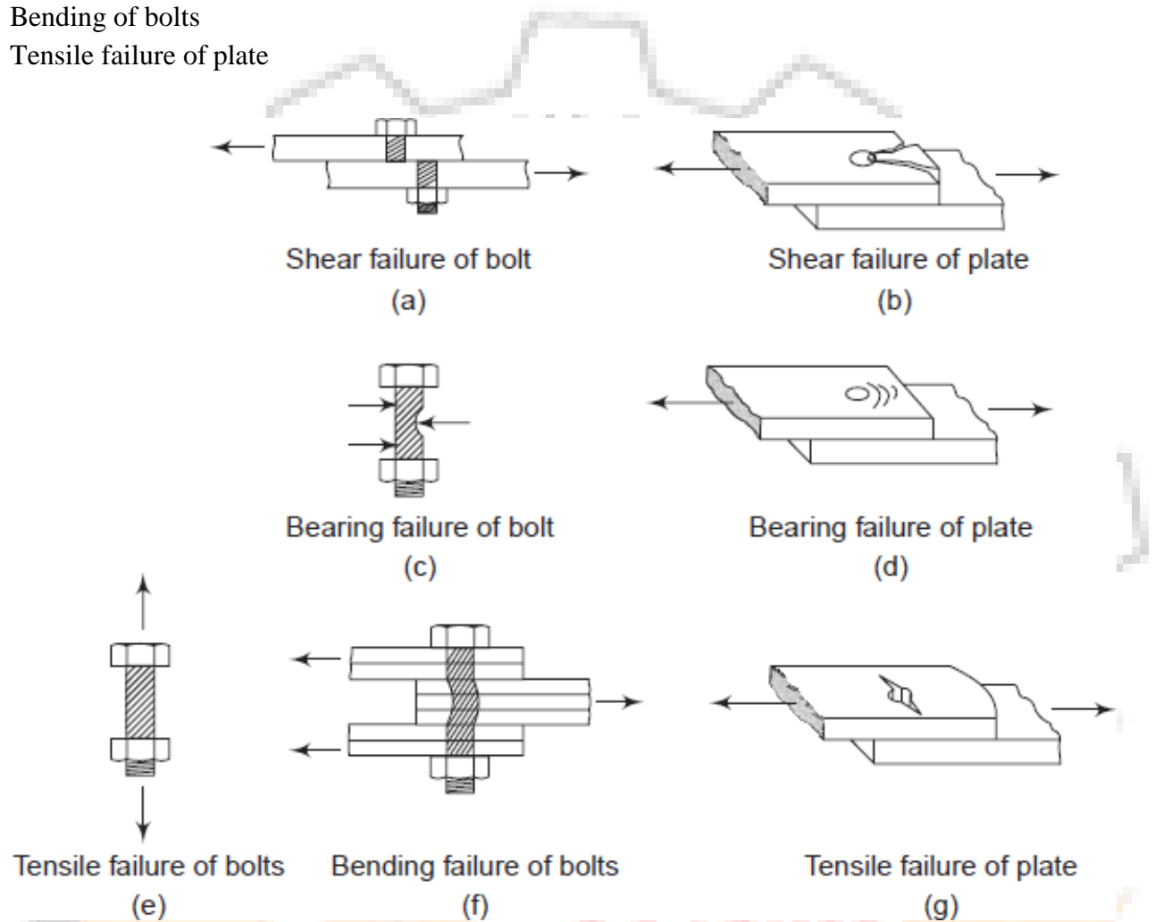
Figure 10.12 Possible failure modes of bolted connections
