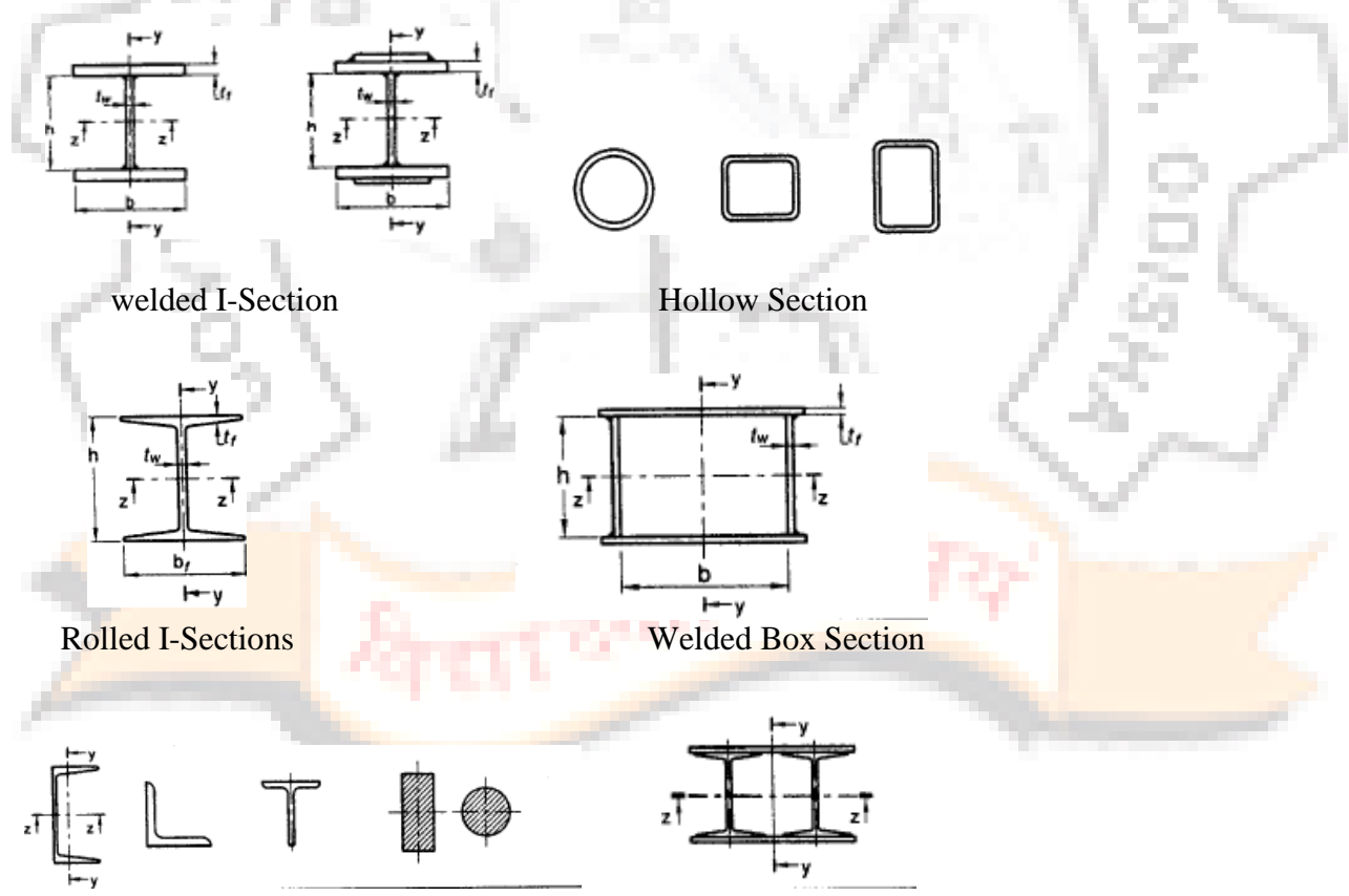
Channel, Angle, T and Solid Sections
