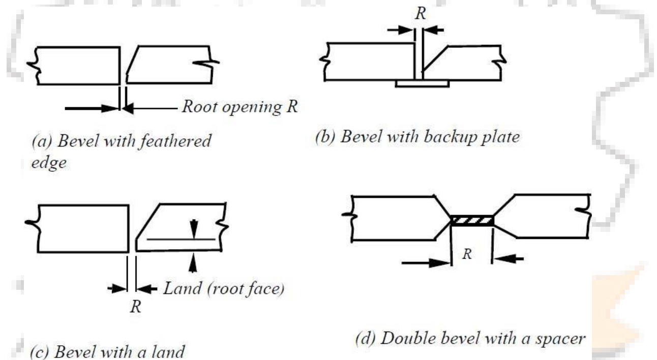
Figure 7.12 Typical edge preparation for butt weld
