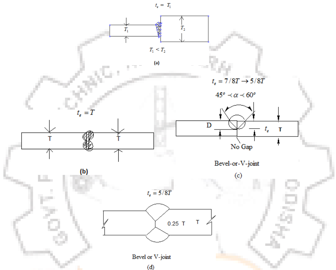
Figure 8.5 Effective throat dimensions for groove welds
