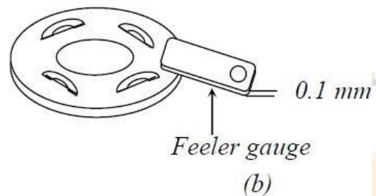
Figure 10.7 Tightening of HSFG bolts
