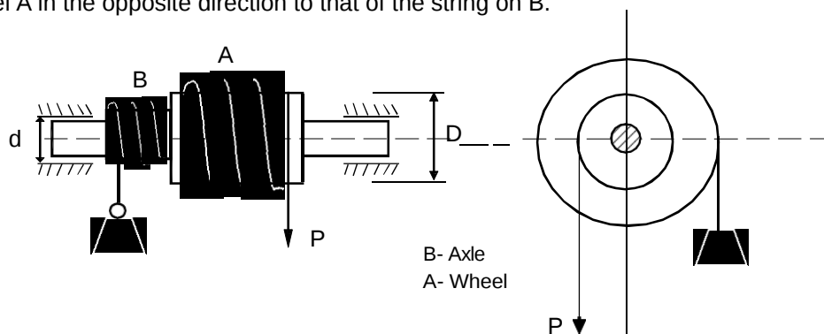
Fig 2.1 Simple wheel and axle
