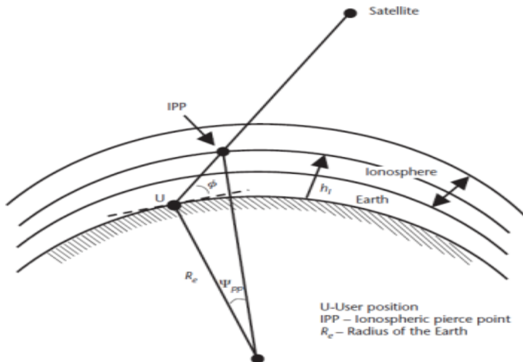
↓ Ionospheric modeling geometry.
